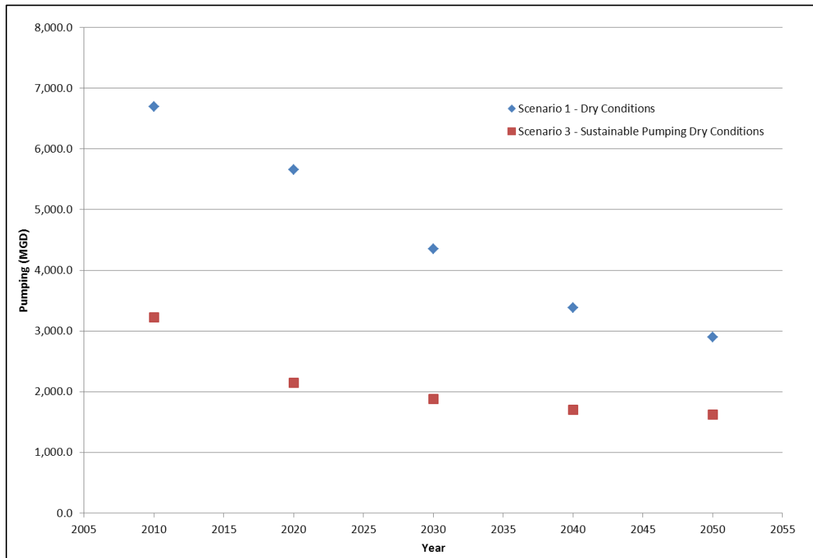
Figure 5-14. Modeled Alluvial Aquifer Well Production for Scenarios 1 and 3
